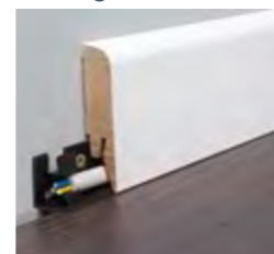
Rounded skirting board
